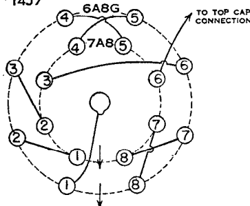
TYPE 7A9 REPLACING TYPE 12A8GT 14B8 14J7
