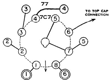
TYPE 7C7* REPLACING TYPE 77 TYPE 7A7* REPLACING TYPE 7B7*
