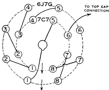
TYPE 7C7* REPLACING TYPE 6J7G TYPE 7L7 TYPE 14C7 REPLACING TYPE 12J7G TYPE 7C7 REPLACING TYPE 12J7G
