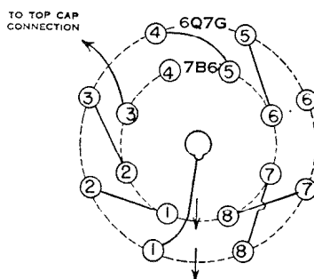
TYPE 7B6 REPLACING TYPE 6Q7GT TYPE 7C6* REPLACING TYPE 12Q7GT TYPE 14B6
