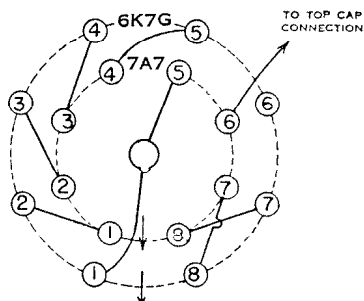
TYPE 7H7 REPLACING TYPE 6K7GT TYPE 7A7 TYPE 14H7 REPLACING TYPE 12K7GT TYPE 14A7
